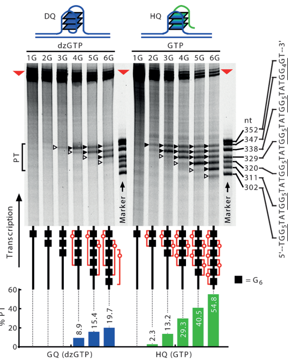
Figure 3. Premature termination (PT) of transcription in plasmids indicates a formation of HQ. Transcription was spiked with 1/20 fluorescein-12-UTP to visualize the transcripts on a denaturing gel. The region between the G-core and terminator was T-free such that PTs can be compared with the full-length transcripts (red arrowhead) without length calibration. The red brackets in the schemes below the gel show combination of G 6 tracts for the formation of DQ or HQ to produce the corresponding PTs (filled arrowheads on gel). Circle indicates positions of major PT. Open arrowheads indicate minor PTs possibly caused by minor HQ structures with a 3/1 (left half gel) or 1/3 (right half gel) DNA/RNA G-tract combination. Graph at the bottom shows PT as % of the total transcripts. Sizes of markers are at the right side of the gel.
